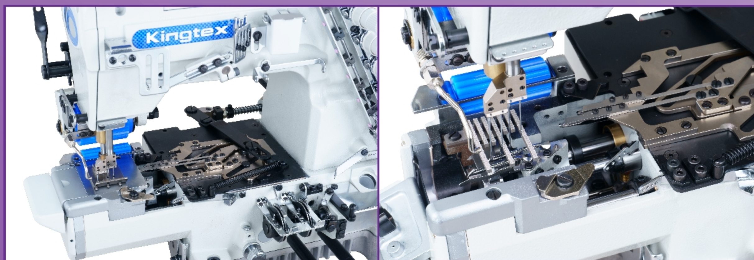
UCP-M2: 氣動式自動切線裝置 Pneumatic Type Top And Bottom Thread Trimming System
