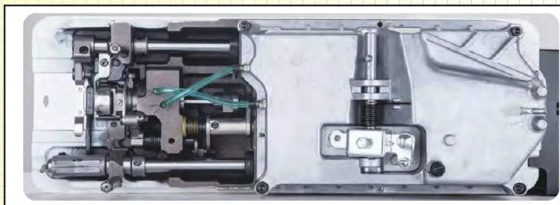
▲ 新型電子鬆線器，比傳統的夾線器，反應更靈敏，精度更高。（避免鬆線不回覆，傳動鋼絲易斷） Brand new design of electronic type thread tension disc. reaction faster than traditional type thread tension disc. (Thread tension release non-retrieval situation and easy broken transmission wire can be avoided)
