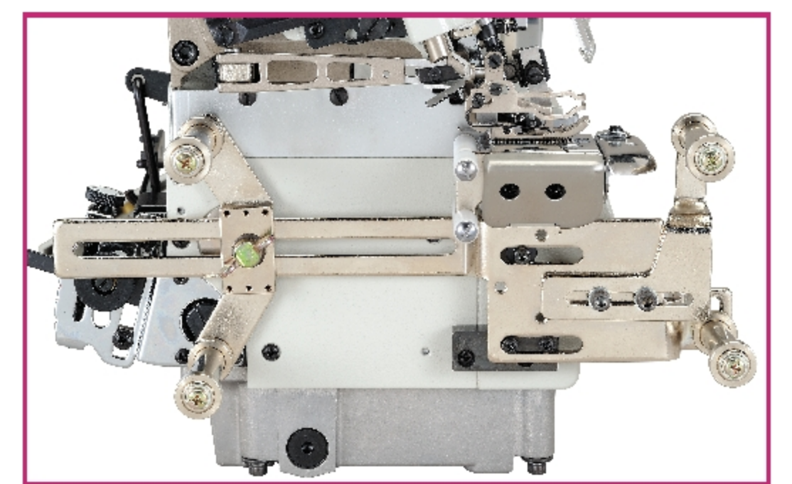
筒型衣物撐開滾輪組 (TR012) FABRIC TENSION CONTROLLING DEVICE 可依衣物長短配合選用。TR012 適用範圍 500 ~ 800 mm。 (TENSION ROLLER) Can be used for different lengths of garments Suitable length: 500 ~ 800 m.m.
