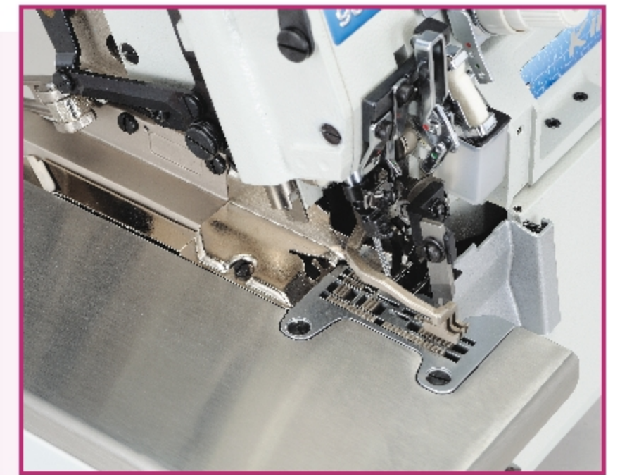
US040:側吸風式自動切線刀(水平吸風式) Side suction type thread trimmer (horizontal type).
