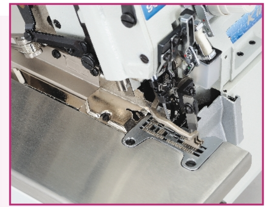
US040:側吸風式自動切線刀(水平吸風式) Side suction type thread trimmer (horizontal type).
