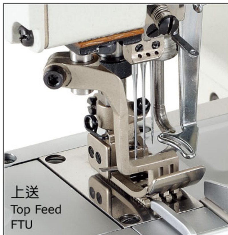
直驅 Direct-Drive FTD/FTU
