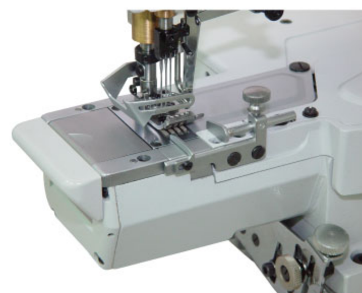
CT9011(280mm)
